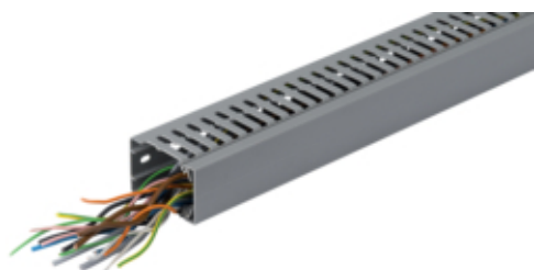
slottet panel trunking BA7A 60x40, grey
