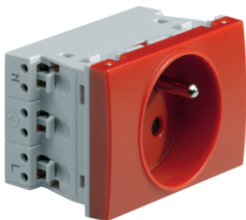
Systo Socket 2P+T 16A for trunking Red
